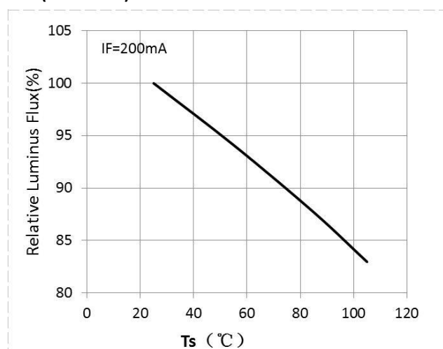
Fig 5. Ambient Temperature vs. Relative Luminous flux ( I_F=200\text{mA} )
