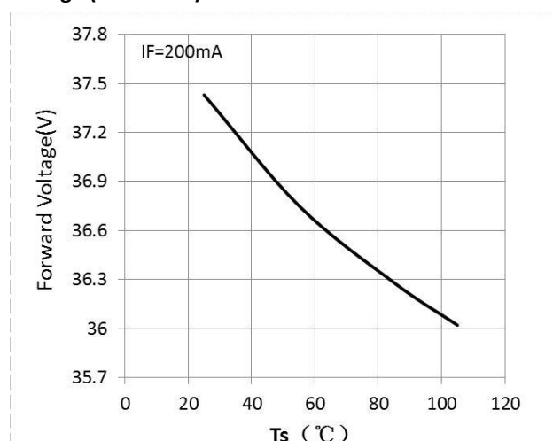
Fig 6. Ambient Temperature vs. Relative Forward Voltage ( I_F=200\text{mA} )
